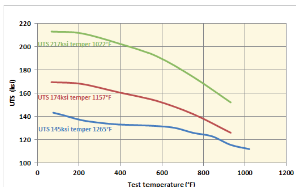
Evolution of hot properties of GKH for different tempering treatments
