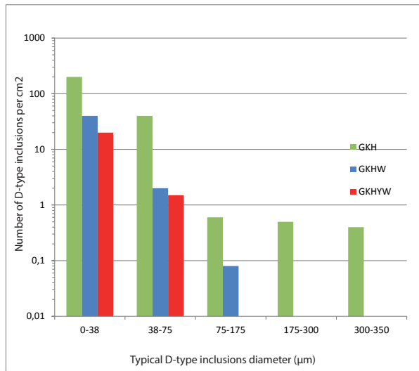
D-type inclusions Typical value number vs diameter
