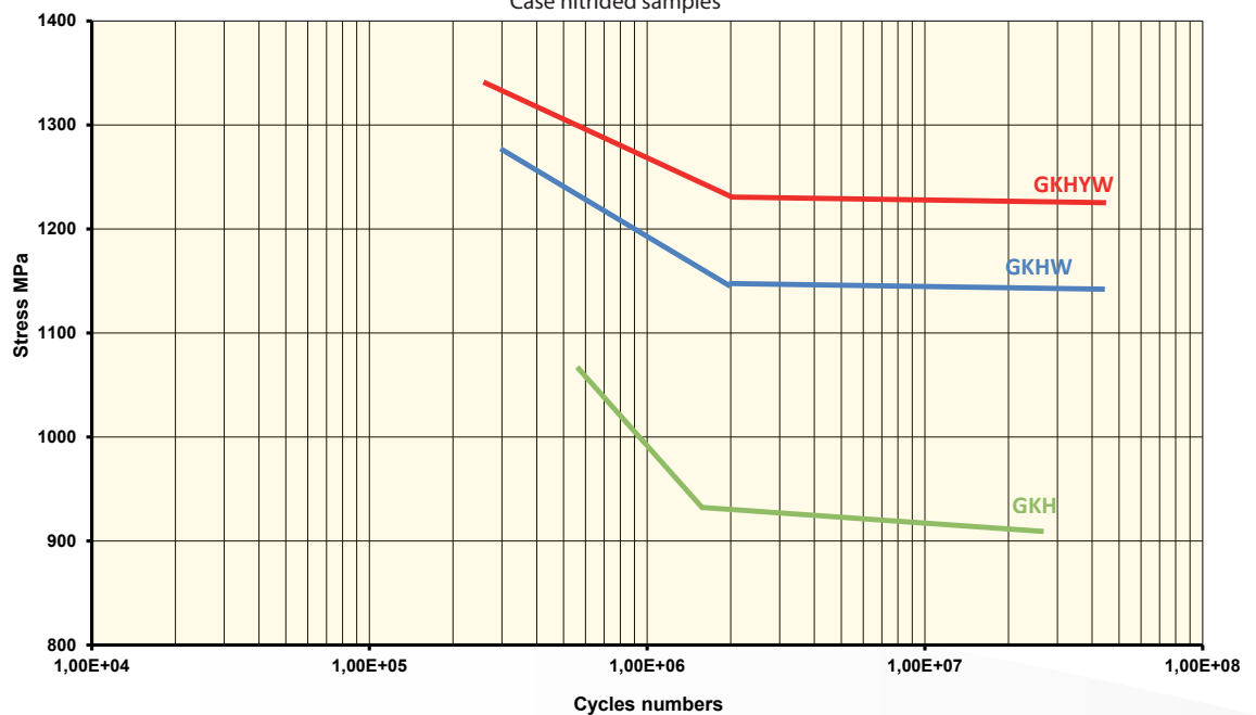
S-N curve - rotative bending mode Target UTS 1250MPa, 181ksi / temper 620°C, 1148°F Case nitrided samples
