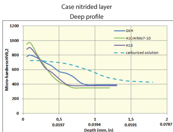
Typical case hardened profiles after gas nitriding : low depth profile 0.25mm, 0.0098in and deep profile 0.7mm, 0.0276in for GKH
